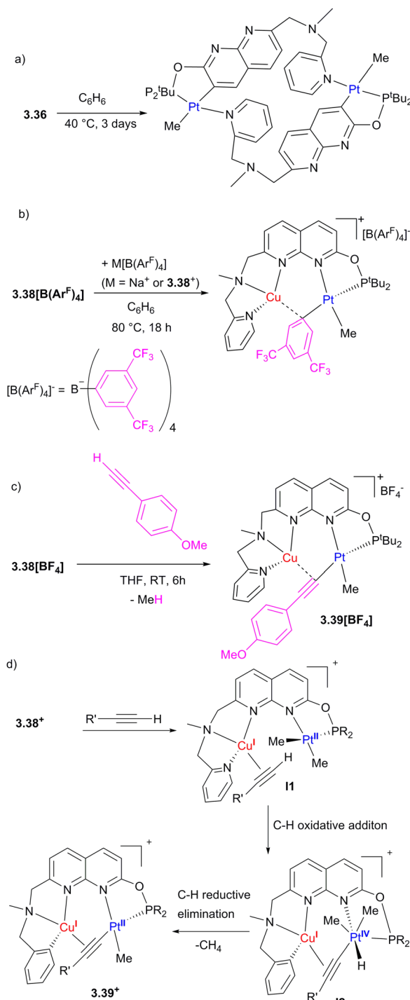
Scheme 31 Reactivity of Pt/Cu complexes: (a) rollover cyclometallation of a monometallic 3.36. (b) Aryl group transfer from the [B(Ar^F)_4]^- ( B(Ar^F)_4 = tetrakis[3,5-bis(trifluoromethyl)phenyl]borate) to 3.38 + . (c) Reactivity of 3.38 + with a terminal alkyne. (d) Proposed mechanism of alkyne activation by 3.38 + .
