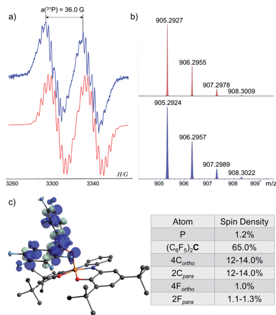
Fig. 7 (a) EPR spectra of [1\text{-OC}(\text{C}_6\text{F}_5)_2]^\bullet (blue) and its simulation (red); (b) MS of the reduced [1\text{-OC}(\text{C}_6\text{F}_5)_2]^\bullet ( 905.2927 (M) ^\bullet ) (red) and its simulation (blue); (c) DFT calculated Mulliken atomic spin densities in [1\text{-OC}(\text{C}_6\text{F}_5)_2]^\bullet .
