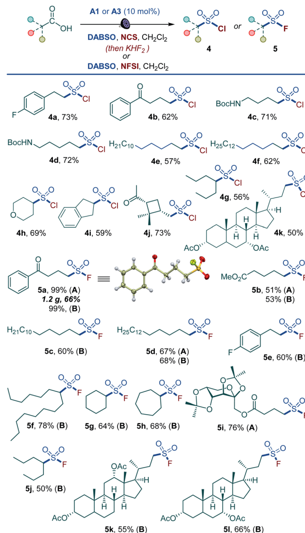
Scheme 3 Scope of the direct decarboxylative chloro- and fluoro-sulfonylation. Reaction conditions: carboxylic acid (0.3 mmol), DABSO (0.33–0.36 mmol), A1 (10 mol%), N -chlorosuccinimide (NCS) (0.6–0.75 mmol), CH 2 Cl 2 (6 mL), LED light (400 nm), 8–12 h, then purification for 4, or (method A) 2 M KHF 2 (0.35 mL, 0.69 mmol), MeCN (2 mL), 50 °C, 3 h or 80 °C, 5 min. Method B: carboxylic acid (0.3 mmol), DABSO (0.45 mmol), A2 (10 mol%), N -fluorobenzenesulfonimide (NFSI) (0.45 mmol), CH 2 Cl 2 (6 mL), LED light (400 nm), 12 h.
