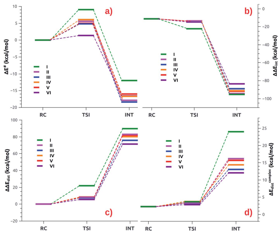
Fig. 6 (a) ASM diagrams for the electronic energy variation ( \Delta E ) along the reaction path connecting RC, TSI and INT structures for complexes [ ^t\text{Bu}_3\text{PAuI} ]–[ ^t\text{Bu}_3\text{PAuVI} ]. (b) ASM diagrams for the variation of the interaction energy stabilization ( \Delta\Delta E_{\text{int}} ) along the reaction path connecting RC, TSI and INT structures for complexes [ ^t\text{Bu}_3\text{PAuI} ]–[ ^t\text{Bu}_3\text{PAuVI} ]. (c) ASM diagrams for the overall variation of the distortion energy penalty ( \Delta\Delta E_{\text{dist}} ) along the reaction path connecting RC, TSI and INT structures for complexes [ ^t\text{Bu}_3\text{PAuI} ]–[ ^t\text{Bu}_3\text{PAuVI} ]. (d) ASM diagrams for the penalty due to the distortion of the complex ( \Delta E_{\text{complex}}^{\text{dist}} ) along the reaction path connecting RC, TSI and INT structures for complexes [ ^t\text{Bu}_3\text{PAuI} ]–[ ^t\text{Bu}_3\text{PAuVI} ]. Results for [ ^t\text{Bu}_3\text{PAuI} ] and [ ^t\text{Bu}_3\text{PAuII} ] have been taken from ref. 33 and 45, respectively.
