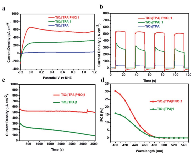
Fig. 6 (a) Linear sweep voltammograms for TiO 2 |TPA|PNO| 1 (red), TiO 2 |TPA| 1 (green) and TiO 2 |TPA (blue) under 1 sun illumination in pH = 7, 0.1 M phosphate buffer containing 0.4 M NaClO 4 . (b) Photocurrent density–time traces over 15 s dark–light cycles for the three photoanodes at a constant bias of 0.4 V vs. NHE. (c) Photocurrents for TiO 2 |TPA|PNO| 1 (red) and TiO 2 |TPA| 1 (green) at a constant bias of 0.4 V vs. NHE under continuous 1 sun illumination. (d) Incident photon-to-current efficiencies (IPCEs) for TiO 2 |TPA|PNO| 1 (red) and TiO 2 |TPA| 1 (green) at 0.4 V vs. NHE.
