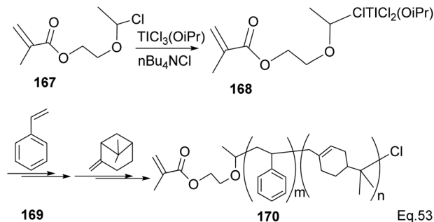
Scheme 47 Ti(iOPr) 3 Cl 3 -promoted cationic copolymerization of β-pinene and styrene.
