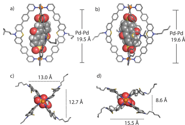
Fig. 3 Two conformational isomers in the crystal structure of the host-guest assembly [G1@1] 2+ : conformer A (HG-A, left) and conformer B (HG-B, right), in side view along the Pd-Pd axis (a and b), and downward the Pd-Pd axis (c and d) (hydrogen substituents, solvent molecules and other G1 anions are omitted for clarity).
