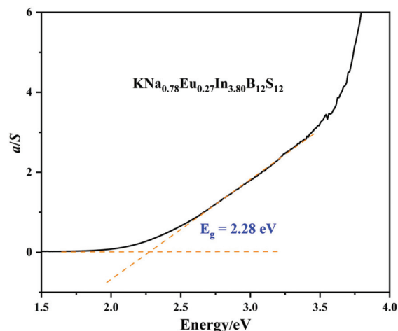
Fig. 6 UV-vis-NIR diffuse reflectance spectrum of 1 .
