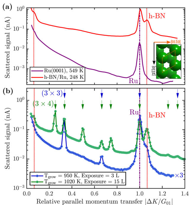
Fig. 2 (a) Comparison of the angular diffraction scans for clean Ru(0001) in purple and the completed h-BN overlay on Ru in red. The [0110] scanning direction ( \vec{\Gamma M} ) is shown in the inset. The purple dash-dotted line indicates the position of the first order Ru diffraction peak and the red dotted lines the h-BN Moiré peaks. (b) Diffraction scans during borazine exposure reveal additional superstructures, depending on the growth temperature and total exposure. The position (shown by the arrows at the top) and spacing of the additional peaks reveal a (3 \times 3)/(3 \times 4) superstructure plotted in blue/green. Low exposure at lower temperatures reveals a (3 \times 3) structure (blue curve, grown at 950 K), while at higher exposures and higher temperatures an intermediate (3 \times 4) pattern emerges (green curve, grown at 1020 K). To improve the signal to noise ratio, the sample was subsequently cooled down for the duration of both scans and the blue curve was scaled by a factor of 3 to facilitate comparison.
