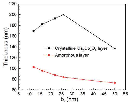
Fig. 7 The thicknesses of crystalline \text{Ca}_3\text{Co}_4\text{O}_9 and amorphous layers in porous films obtained by annealing \text{Ca(OH)}_2/\text{Co}_3\text{O}_4 multilayers created from \text{CaO}/\text{Co}_3\text{O}_4 multilayers with 12 \leq b_t \leq 50 nm.
