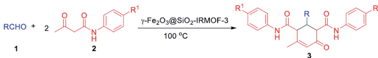
Fig. 30 Synthesis of cyclohexenone derivatives using \gamma-Fe_2O_3@SiO_2/IRMOF-3 catalyst. This figure was adapted with permission from Journal of Catalysis , 2020, 387, 39–46. 188
