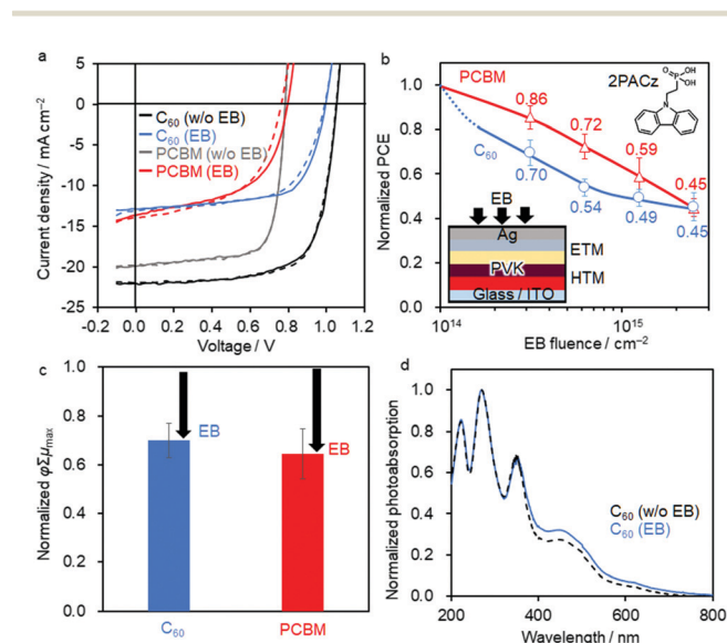
Fig. 1 (a) JV curve of the best-performing inverted PSCs of Device 2 (ITO/2PACz/PVK/C 60 /BCP/Ag) and Device 3 (ITO/PEDOT:PSS/PVK/PCBM/PDINO/Ag) with (blue and red curves) and without EB exposure (black and grey curve, F_{\text{EB}} = 2.5 \times 10^{15} \text{ cm}^{-2} ). The solid and dashed lines are the reverse and forward scans, respectively. (b) Decrease in the PCE upon EB irradiation normalized by each initial PCE. Average values are superimposed. Schematic shows the device structure and EB irradiation geometry. The chemical structure of 2PACz is superimposed. (c) \phi\Sigma\mu_{\text{max}} of TRMC transients normalized by that of the as-prepared C 60 or PCBM layer ( \lambda_{\text{ex}} = 355 \text{ nm} , I_0 = 7.0 \times 10^{15} \text{ photons cm}^{-2} \text{ pulse}^{-1} ). The arrows represent the change from the original value without EB irradiation. (d) Normalized photoabsorption spectra of a C 60 film before (black line) and after EB exposure (blue line, F_{\text{EB}} = 2.5 \times 10^{15} \text{ cm}^{-2} ).
