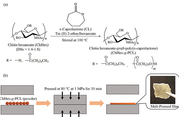
Fig. 14 (a) Surface-initiated ring-opening graft polymerization of ε-caprolactone (CL) from chitin hexanoates (ChHex) to obtain chitin hexanoate-graft-poly(ε-caprolactone) (ChHex-g-PCL), and (b) melt-pressing experiment of ChHex-g-PCL (reprinted with permission from ref. 121. Copyright 2022 Elsevier; DOI: 10.1016/j.carbpol.2021.119024).
