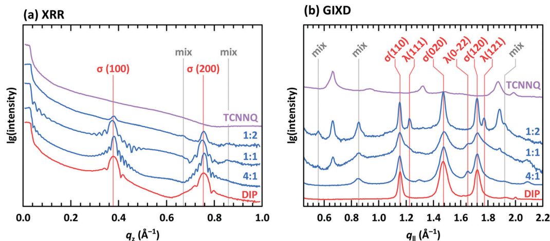
Fig. 8 (a) X-ray reflectivity (XRR) and (b) grazing incidence X-ray diffraction (GIXD) measurements for single component and co-deposited films of DIP and TCNNQ. The peaks denoted as \sigma(\lambda) are related to phases containing upright standing (lying) DIP molecules. Peaks marked as "mix" are attributed to the formed mixed crystal. Corresponding respective reciprocal space maps are shown in ESI† (see Fig. S1).
