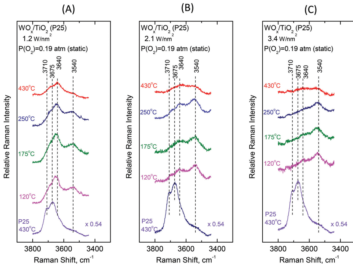
Fig. 10 \text{WO}_x/\text{TiO}_2 (P25) with surface density of (A) 1.2 \text{ W nm}^{-2} ; (B) 2.1 \text{ W nm}^{-2} ; and (C) 3.4 \text{ W nm}^{-2} . Sequential Raman spectra at static equilibrium under p_{\text{O}_2} = 0.19 \text{ atm} at temperatures as indicated by each spectrum. Each panel includes the Raman spectrum of pure \text{TiO}_2 (P25) at 430^\circ\text{C} as reference. Spectral parameters: \lambda_0 = 532.0 \text{ nm} ; laser power, w = 20 \text{ mW} ; and resolution, 2 \text{ cm}^{-1} .
