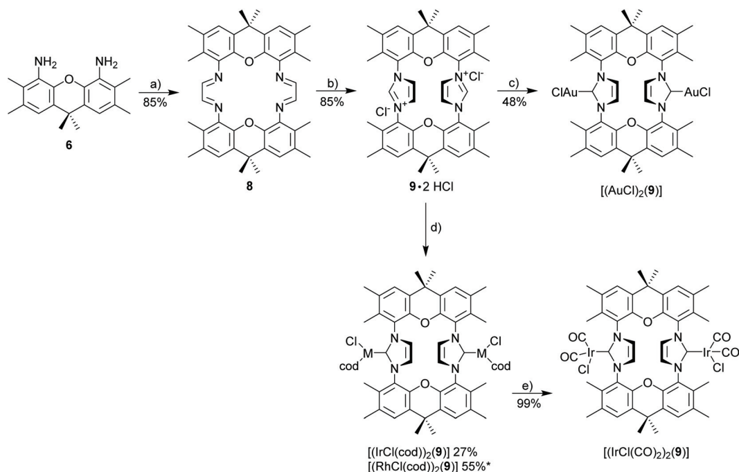
Scheme 3 Synthesis of azolium salt 9 ·2HCl and derived metal complexes. Reagents and conditions: (a) glyoxal, p\text{TsoH} , n\text{BuOH} , 50 °C; (b) paraformaldehyde, \text{Me}_3\text{SiCl} , \text{EtOAc} , 70 °C, 24 h; (c) \text{Ag}_2\text{O} , \text{MeOH} , rt, 24 h then [\text{AuCl}(\text{SMe}_2)] , 50 °C, 2 h; (d) [\text{MCl}(\text{cod})_2] ( \text{M} = \text{Ir}, \text{Rh} ), sodium amylate, THF, -78 °C; (e) \text{CO} , 0 °C, \text{CH}_2\text{Cl}_2 30 min; (* yield of crude complex).
