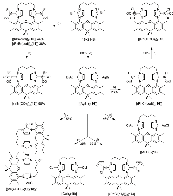
Scheme 7 Synthesis of metal complexes with NHC 16 . Reagents and conditions: (a) \text{Ag}_2\text{O} , MeOH, rt, 24 h; (b) [\text{RhCl}(\text{cod})]_2 , 50^\circ\text{C} , 2 h; (c) [\text{AuCl}(\text{SMe}_2)] (2.0 eq.), 50^\circ\text{C} , 2 h; (d) [\text{PdCl}(\text{allyl})]_2 , DCM, rt, 24 h; (e) CuI, DCM, rt, 24 h; (f) [\text{AuCl}(\text{SMe}_2)] (1.5 eq.), 50^\circ\text{C} , 2 h; (g) [\text{MCl}(\text{cod})]_2 (M = Ir, Rh), \text{K}_2\text{CO}_3 , NaOAc, KBr, MeCN, 80^\circ\text{C} , 12 h; (h) CO, 0^\circ\text{C} , \text{CH}_2\text{Cl}_2 , 30 min.
