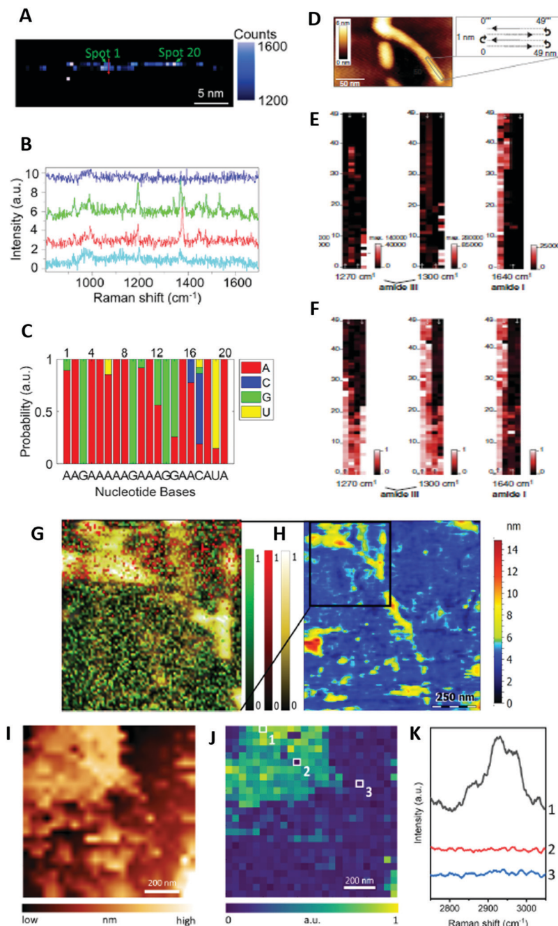
Fig. 4 (A–C) TERS of RNA: (A) TERS image plotting the integral intensity of the TERS peak at 1370 cm -1 attributed to A, G, U and C nucleobases (0.5 nm scanning step size); (B) four TERS spectra along the red arrow drawn in panel A; (C) measured sequence from spot 1 to spot 20 along the strand drawn in panel A, with the most probable bases labelled at the bottom. This sequence is globally consistent with the genuine RNA sequence AAGAAAAGAAAGGAUCCUA, except at spots 16 and 18 where an A nucleobase is identified instead of U and C, respectively. Adapted with permission from Z. He et al. , ACS Photonics , 2021, 8 , 424–430. Copyright (2021) American Chemical Society. (D–F) TERS of an insulin amyloid fibril: (D) AFM topography image of a fibril; (E) TERS maps of the region indicated in panel D from fitted amide I and amide III band intensities, with pixel brightness proportional to band intensity (1 nm scanning step size); (F) corresponding TERS maps obtained from a SUA analysis. Adapted with permission from T. Deckert Gaudig et al. , Sci. Rep. , 2016, 6 , 33575. Copyright (2016) Springer Nature Group. This work is licensed under the Creative Commons Attribution 4.0 International Licence ( https://creativecommons.org/licenses/by/4.0/ ). (G and H) TERS of Aβ 1-42 aggregates: (G) distribution of TERS spectra indicating the presence of mainly unstructured coils/turns (green), antiparallel β-sheet (red) and parallel β-sheet (yellow) secondary structures in a representative sample, containing various Aβ 1-42 aggregates (~6 nm scanning step size). The distributions of normalised values of the Pearson correlation coefficients between three marker TERS spectra are represented and superimposed on the AFM topography image. (H) Overview AFM topography of the same sample. Adapted with permission from E. Lipiec et al. , Angew. Chem., Int. Ed. , 2021, 60 , 4545–4550. Copyright (2021) Wiley-VCH GmbH. (I–K) TERS of a DPPC supported lipid monolayer: (I) STM topography image of a DPPC monolayer region; (J) TERS image of the C–H stretching intensity measured in the area shown in panel I (40 nm scanning step size); TERS spectra measured at locations 1–3 marked in panel J. No TERS signal is observed at position 3 (outside the DPPC monolayer) and position 2 that corresponds to a nanoscale hole in the DPPC monolayer. Adapted with permission from Y. Pandey et al. , Angew. Chem., Int. Ed. , 2021, 60 , 19041–19046. Copyright (2021) Wiley-VCH GmbH.
