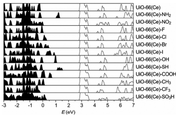
Fig. 7 HSE06 calculated DoS of functionalised UiO-66(Ce). The conduction band minima are aligned. Reprinted with permission from ref. 128. Copyright (2018) American Chemical Society.
