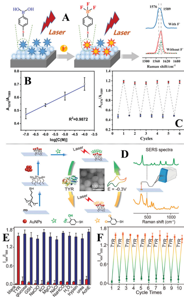
Fig. 20 (A) Schematic illustration of the working principles of the pH-reversible F - sensor; (B) plot showing the average area ratio between the SERS peak at 1576 cm -1 and 1589 cm -1 as a function of the log concentration of F - ; (C) plot showing the SERS activity of the sensor after 6 cycles of regeneration; (D) schematic illustrations of the fabrication of the electro-reversible tyrosinase sensor. Inset shows a SEM image of the enhancing Au nanoparticles on the surface of the sensor; (E) bar chart showing the ratio between the SERS intensity of the vibration bands at 484 cm -1 and 588 cm -1 as a function of sample type. The red histograms correspond to the signals obtained from blank reference samples and pure samples of the chemicals labelled below. The blue histograms correspond to samples containing a mixture of tyrosinase and the chemicals labelled below. The error bars represent the standard deviation calculated from 3 independent measurements; (F) plot showing the SERS activity of the sensor after 10 cycles of electro-regeneration. Panel (A–C) reproduced with permission from ref. 272, copyright 2019 American Chemical Society. Panel (D–F) reproduced with permission from ref. 273, copyright 2019 American Chemical Society.
