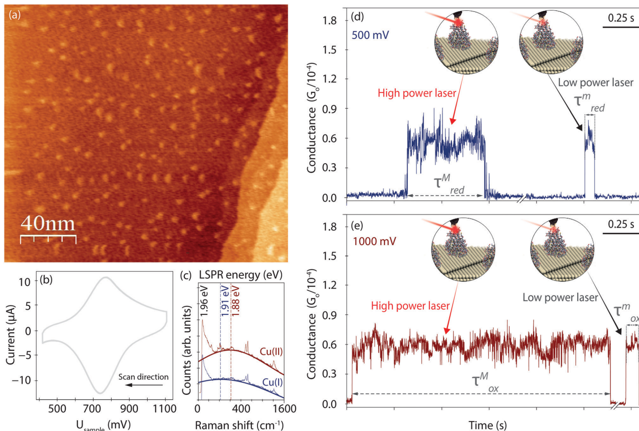
Fig. 2 (a) EC-STM image ( 200\text{ nm} \times 200\text{ nm} , z -scale = 1\text{ nm} ) of an Azu-functionalized Au(111) surface in 50\text{ mM NH}_4\text{Ac} buffer at pH 4.55 with U_{\text{sample}} = 1000\text{ mV} , U_{\text{bias}} = 300\text{ mV} , I_t = 1\text{ nA} . (b) CV of Azu under the conditions of (a) with a scan rate of 50\text{ mV s}^{-1} . (c) Raw TER spectra obtained with ca. 9.49\text{ mW } \mu\text{m}^{-2} farfield power density at 1.96\text{ eV} excitation energy and 120\text{ s} integration time of oxidized Cu(II) ( U_{\text{sample}} = 1000\text{ mV} , red) and reduced Cu(I) ( U_{\text{sample}} = 500\text{ mV} , blue) Azu, respectively. LSPR mode energies as extracted from Lorentzian fits to the TER spectral background are indicated with dotted vertical lines. (d and e) Examples of EC-PBJ captures of Azu junctions at (d) U_{\text{sample}} = 500\text{ mV} (blue, \tau_{\text{red}}^M ) and (e) U_{\text{sample}} = 1000\text{ mV} (red, \tau_{\text{ox}}^M ) with maximum ( \tau^M ) and minimum ( \tau^m ) laser power conditions of 9.49\text{ mW } \mu\text{m}^{-2} and 6.72 \times 10^{-2}\text{ mW } \mu\text{m}^{-2} , respectively.
