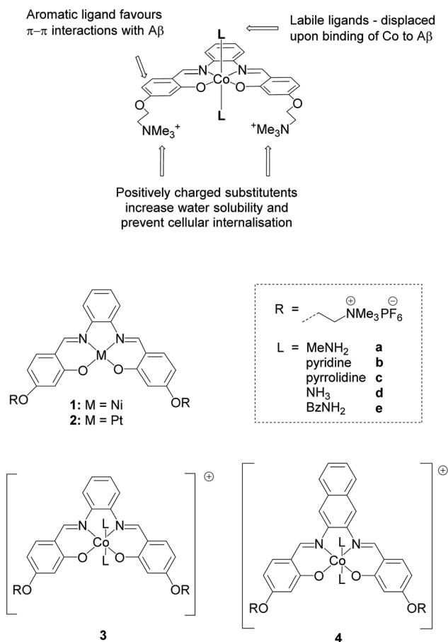
Fig. 1 Structures of metal salphen (1, 2 and 3a–3e) and salnaph (4a–4e) investigated.
