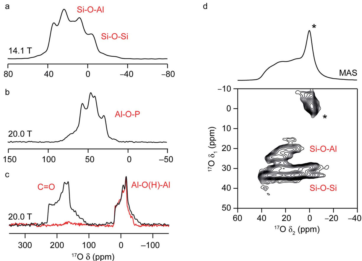
Fig. 3 ^{17}\text{O} MAS NMR spectra of (a) aluminosilicate CHA zeolite, (b) calcined CHA-type aluminophosphate framework, SIZ-4 and (c) calcined ALMIL-53. The external field strengths at which spectra were recorded are shown in the figure. In (c), the ^1\text{H} - ^{17}\text{O} CP MAS NMR spectrum is shown in red. (d) ^{17}\text{O} (14.1 T) MAS and MQMAS of a hydrated CHA zeolite (after slurring with \text{H}_2^{17}\text{O}(\text{l}) ).
