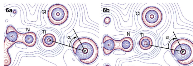
Fig. 8 Contour map of \nabla^2\rho in the \text{P}_c\text{–Ti–Cl} plane for 6a and 6b (red lines indicate charge concentration and blue lines indicate charge depletion).
