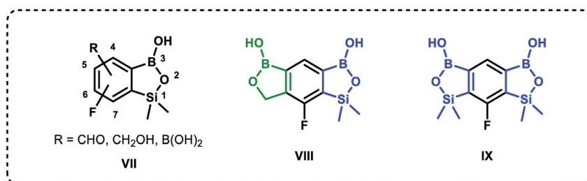
Fig. 2 Examples of functionalized benzosiloxaboroles. 26 Position numbering scheme is additionally provided for the general structure VII (note that it is different between benzoxa- and benzosiloxaboroles).
