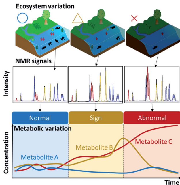
Fig. 3 Conceptual diagram of metabolic profiling using NMR spectra for evaluating homeostasis in ecosystems. Top, the schematic diagram shows collapse of an environmental ecosystem. Middle, the NMR signals of samples from environments can be profiled as a relative intensity change. Bottom, the corresponding variation of three states (normal, sign, and abnormal) are illustrated by hypothetical fluctuations in the concentrations of three metabolites (metabolite A, blue; metabolite B, yellow; and metabolite C, red).
