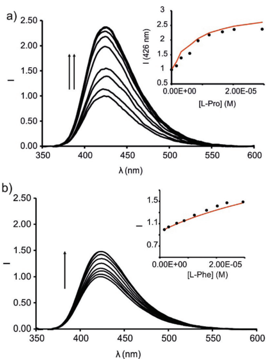
Fig. 9 Emission spectra registered during the competitive IDA experiments of 6 \subset 1in complex (1 \mu\text{M} ) with incremental addition of L-Pro (up to 30 equiv.) (a) and L-Phe (up to 30 equiv.) (b) in dichloromethane solution; \lambda_{\text{exc}} = 335 nm. Insets: plots of the emission change at 426 nm (black circles) vs. concentration of the amino acid. The red line corresponds to the fit of the titration data to a 1 : 1 theoretical binding model considering only two emissive species: the free cavitand and the 1 : 1 complex with the corresponding amino acid.
