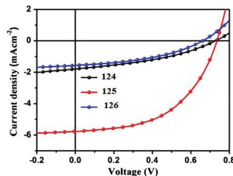
Fig. 22 Current–voltage characteristics of optimized photovoltaic cells based on 124 : PC 61 BM, 125 : PC 61 BM and 126 : PC 61 BM under illumination of AM 1.5, 100 \text{mW cm}^{-2} white light. Reproduced with permission of Elsevier. 74
