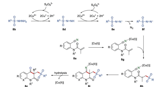
Scheme 8 The construction of sulfonated quinoline-2,4-diones.
