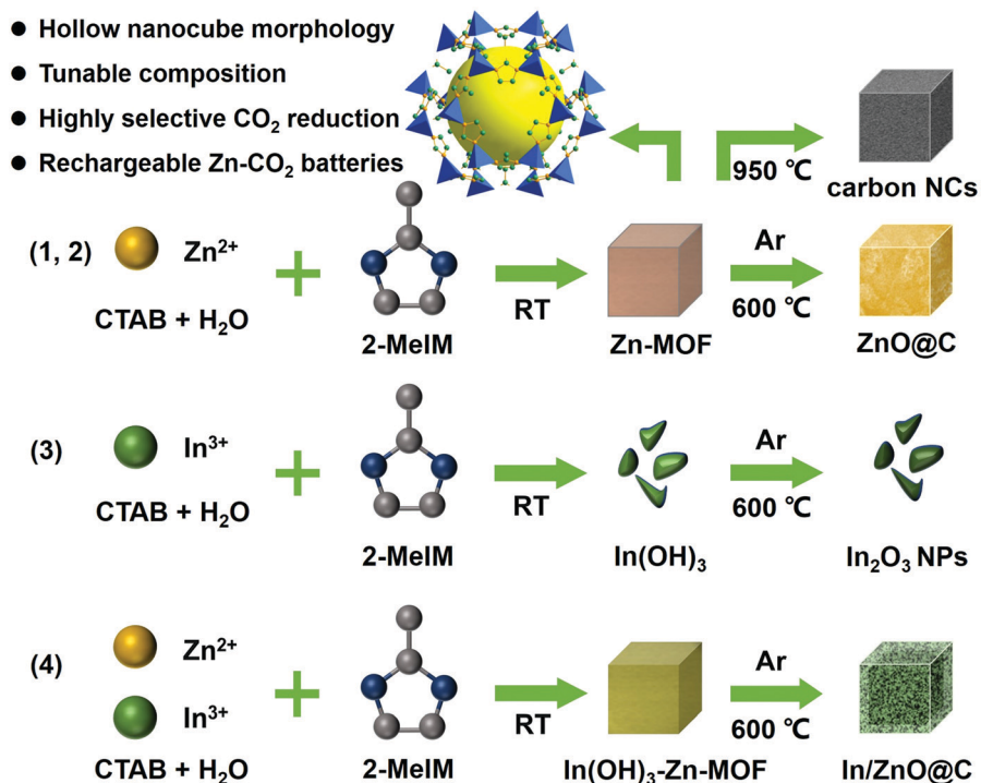
Scheme 1 Schematic illustration of the fabrication of carbon NCs, ZnO@C NCs, In 2 O 3 NPs and In/ZnO@C NCs as CO 2 RR electrocatalysts.
