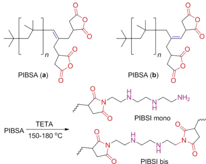
Fig. 4 Bis-succinic anhydride derivatives PIBSA (a) and PIBSA (b), and their triethylenetetramine (TETA) decorated corresponding mono and bis-succinimides (PIBSI mono, PIBSI bis). Reprinted with permission from ref. 77. Copyright 2008, John Wiley and Sons.
