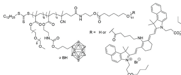
Fig. 4 Structure of the amphiphilic poly(carborane-containing methacrylate)- b -poly(caprolactone) with or without a near-infrared amino-cyanine dye.
