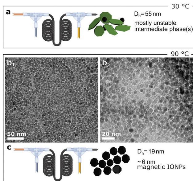
Fig. 4 (a) Schematic of flow synthesis with co-precipitation performed at 30 °C. ( b_{1-2} ) TEM images of IONPs synthesised with co-precipitation performed at 90 °C, D_{\text{TEM}} = 6.1 \pm 0.9 nm. (c) Schematic of flow synthesis with co-precipitation initiated at 90 °C. Fig. S5† shows the particle size distribution. For both temperatures, quenching was performed at 5 s.
