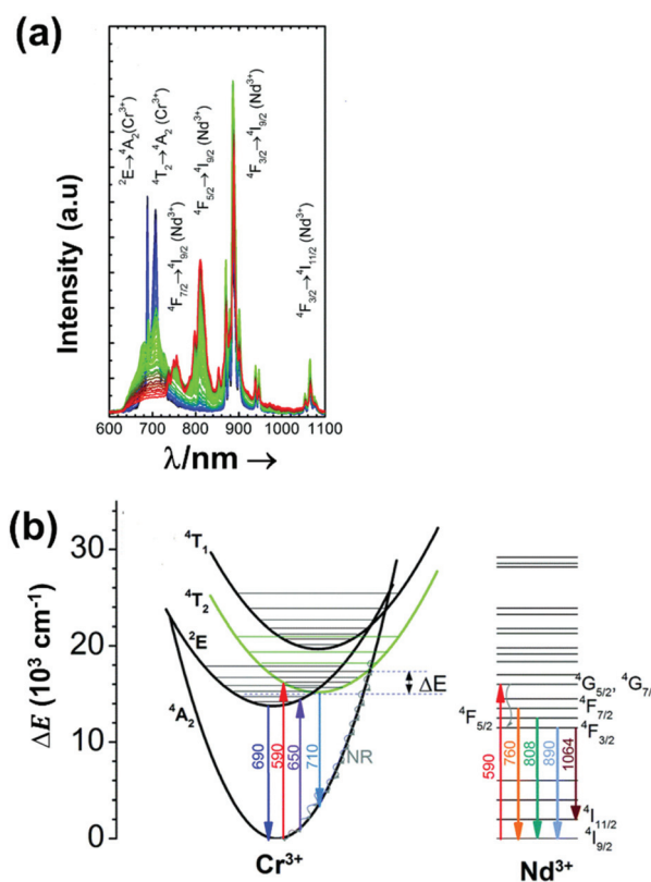
Fig. 16 (a) Emission lines and (b) mechanisms for their generation in Nd^{3+},Cr^{3+} -codoped YAG, after being excited at 590 nm. Reprinted with permission from ref. 155. Copyright 2017, the Owner Societies.
