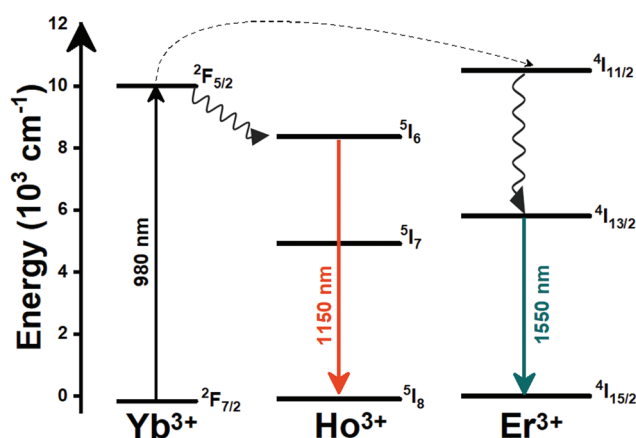
Fig. 34 Mechanism of generation of the emissions lines located in the II- and III-BWs of \text{Er}^{3+}, \text{Ho}^{3+}, \text{Yb}^{3+}:\text{NaYF}_4 nanoparticles under 980 nm excitation.
