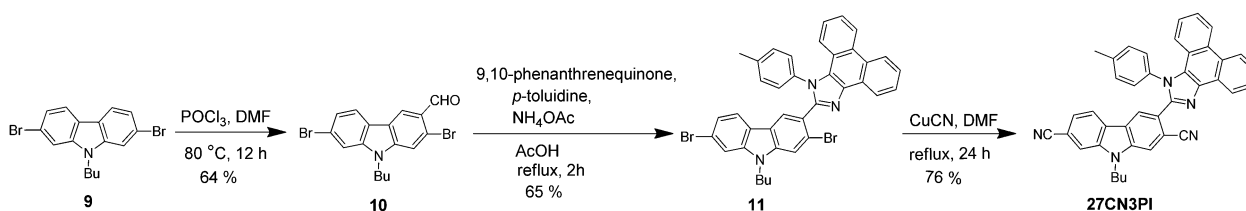
Scheme 2 Synthetic protocol of the dye 27CN3PI .
