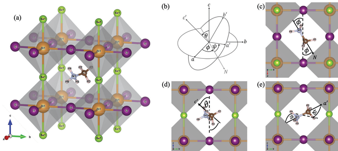
Fig. 1 The cubic structure of \text{CH}_3\text{NH}_3\text{BiSeI}_2 (MABiSeI) with labelled atoms (a); the definition of the Euler angles (b) for the MA cation where the N–C bond is directed to the N-axis. The first rotation is rotated anticlockwise through angle \phi about the c -axis (c). The second rotation is anticlockwise via angle \theta about the a' -axis or N -axis (d). Finally, the third rotation is rotated anticlockwise through angle \psi about the c' -axis (e). Note that all atoms of the inorganic \text{BiSeI}_2 cage were kept fixed throughout the calculations, while the organic MA cation was the only thing to reorient according to the Euler's rotations. Nearly all figures are generated by VESTA. 16
