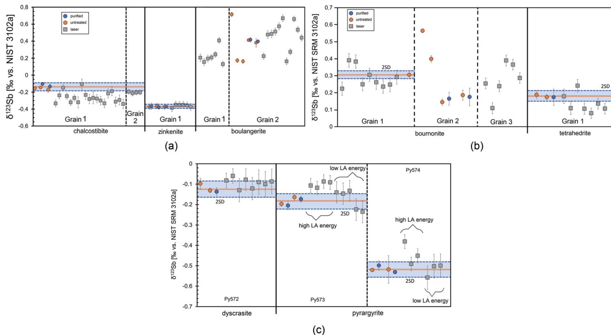
Fig. 6 Comparison of \delta^{123}\text{Sb} values from solution and laser-ablation analysis for: (a) chalcostibite, zinkenite, and boulangerite; (b) bourmonite and tetrahedrite; (c) dyscrasite and pyrargyrite. All LA measurements (squares) were measured relative to SC and recalculated to NIST 3102a. All purified (blue circles) and non-purified (orange circles) solution values are measured and reported relative to NIST 3102a. Error bars for solution represent the 2SD of replicate analyses of the sample, while laser measurement errors are given as 2\sigma (error-propagated internal uncertainties ( 2 SE) of the sample and standard measurements).
