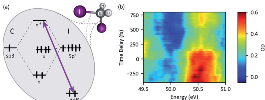
Fig. 9 (a) Term scheme of the diiodomethane ( \text{CH}_2\text{I}_2 ) target molecule. The resonant XUV excitation from the iodine 4d orbital to an antibonding \sigma^* molecular orbital is indicated by the violet arrow. (b) XUV-pump XUV-probe transient absorption spectroscopy of diiodomethane (probe-pulse spectrum).
