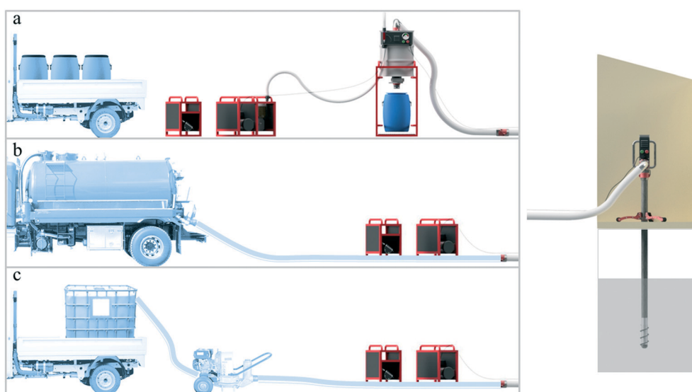
Fig. 4 The Excluder (right) can be linked to a) a custom vacuum system (Flexcreator), b) vacuum truck, or c) a pit-side pump.
