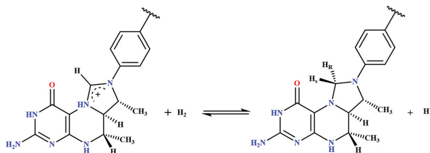
Scheme 24 Scheme of the reversible heterolytic splitting of H 2 by Hmd, showing a hydride stereospecifically transferred into the pro-R site of methenyl-H 4 MPT + to yield methylene-H 4 MPT and a proton.
