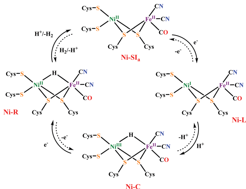
Scheme 23 Proposed catalytic mechanism for reversible H 2 oxidation by [NiFe]-hydrogenases. 367,400
