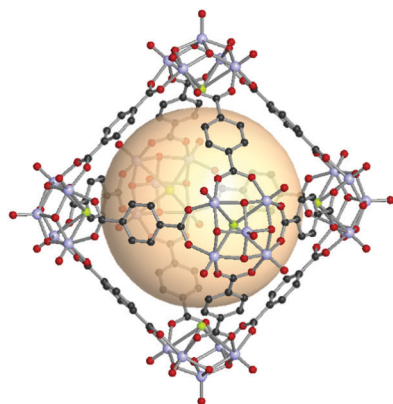
Fig. 12 Structural illustration of VMOP-1 , [\text{V}_5\text{O}_9\text{Cl}]_6(\mathbf{A1})_{12} .
