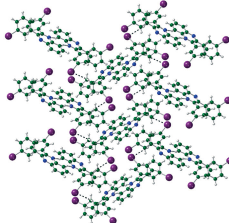
Fig. 5 Formation of sheet structure in \text{Q3,3'I}_2 .
