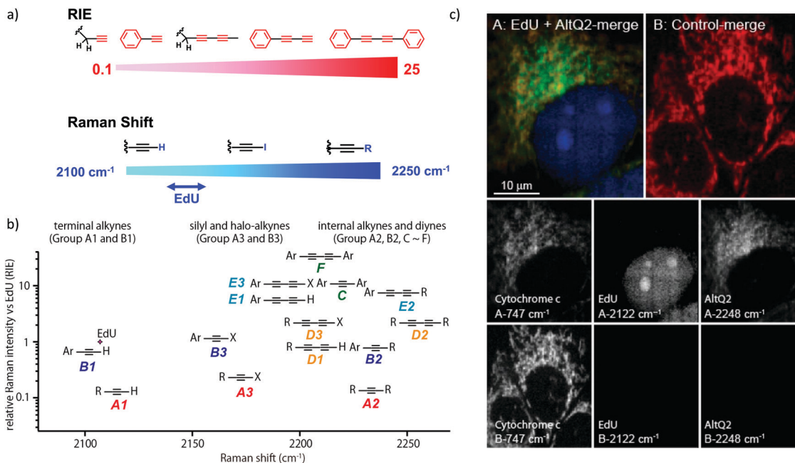
Fig. 3 (a) Raman shift and intensity changes with changes of structure. (b) Plot of relative Raman intensity to EdU vs. Raman shift for various alkynes. (c) Multiplexed ATRI of two alkyne-containing molecules, EdU and AltQ2, in HeLa cells along with untreated control cells. Adapted from ref. 92. Copyright 2012 American Chemical Society.
