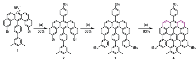
Scheme 1 Synthetic route towards 4 . Reagents and conditions: (a) sodium 2-(4- tert -butylphenyl)acetate, benzoic anhydride, 150 °C, 24 h, 56%; (b) 3- tert -butylphenylboronic acid, \text{Pd}(\text{PPh}_3)_4 , \text{K}_2\text{CO}_3 , \text{H}_2\text{O} , ethanol, toluene, 110 °C, 24 h, 68%; (c) DDQ/ \text{TfOH} , dichloromethane, room temperature, 8 h, 83%. DDQ: 2,3-dichloro-5,6-dicyano-1,4-benzoquinone, \text{TfOH} : trifluoromethanesulfonic acid.
