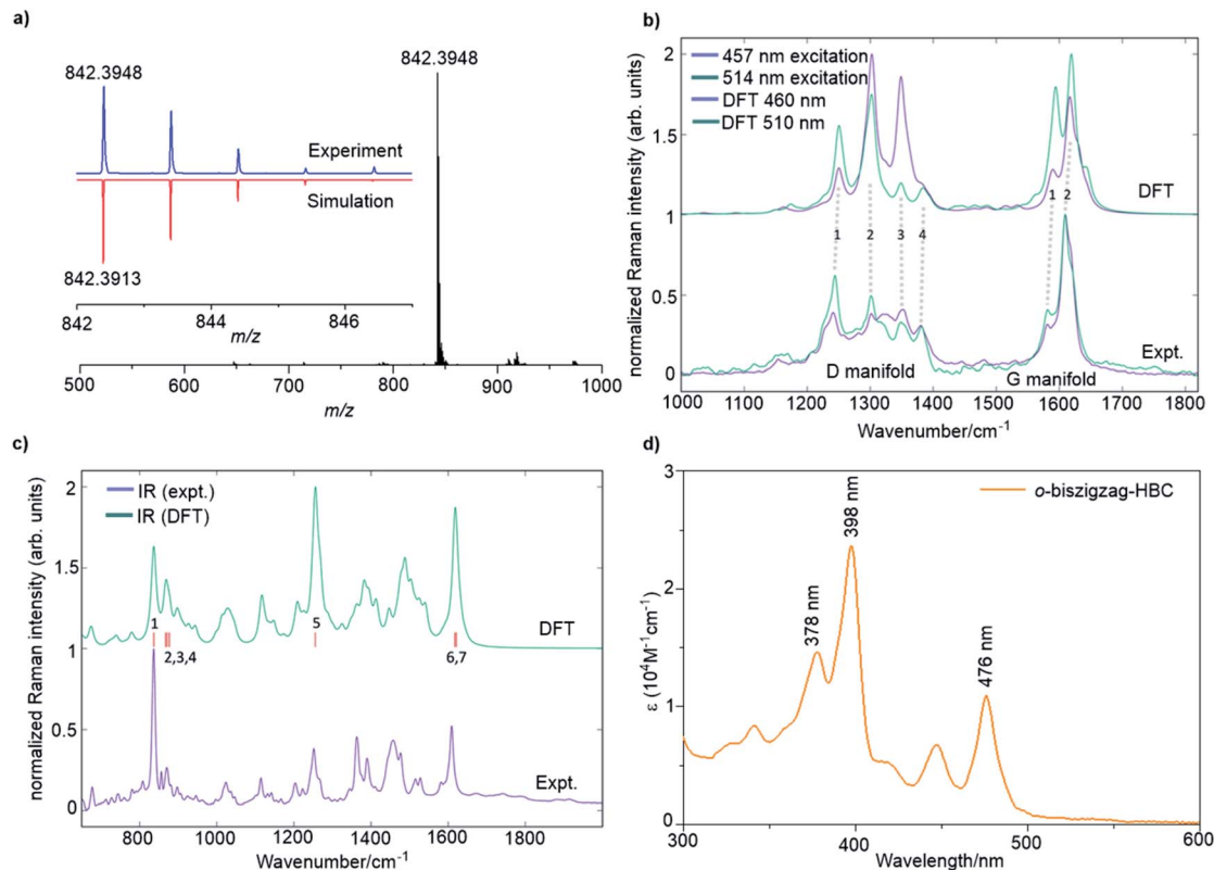
Fig. 2 (a) MALDI-TOF MS of 4 . Inset: isotopic distribution compared with the mass spectrum simulated for \text{C}_{66}\text{H}_{50} . (b) FT-Raman spectra of 4 compared with results from DFT calculations over the D and G regions. (c) Micro FT-IR spectrum of 4 and the simulated spectrum by DFT calculations. (d) UV/vis absorption spectrum 4 in THF. Concentration: 2 \times 10^{-5} M.
