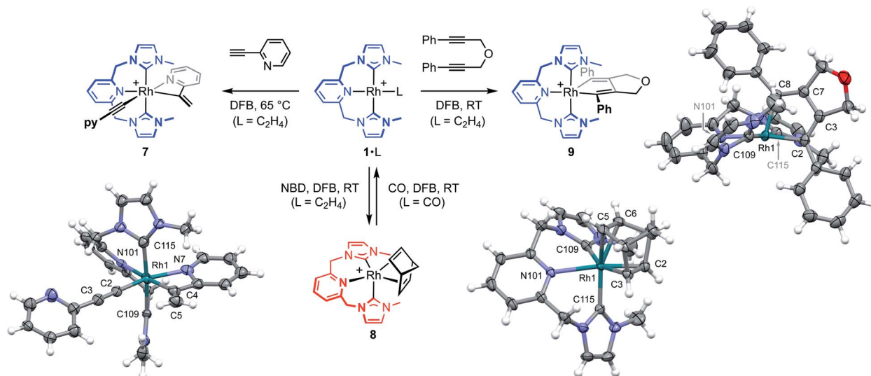
Fig. 5 Reactivity of 1 · C_2H_4 relevant to the proposed mechanism ([ BAR^F_4 ] ^- anions omitted). Solid-state structures of the cations of 7 , 8 and 9 (not unique, Z' = 2 ) shown with 30%, 50% and 50% probability thermal ellipsoids, respectively. Selected data: 7 , Rh1–C2, 1.92(2) Å; C2–C3, 1.21(2) Å; Rh1–C2–C3, 179(2)°; Rh1–C4, 2.02(2) Å; C4–C5, 1.30(3) Å; Rh1–N7, 2.15(2) Å; Rh1–C4–C5, 140(2)°; Rh1–N101, 2.25(2) Å; Rh1–C109, 2.01(2) Å; Rh1–C115, 2.01(2) Å; C109–Rh1–C115, 174.5(8)°; 8 , Rh1–Cnt(C2,C3), 1.964(2) Å; Rh1–Cnt(C5,C6), 2.144(2) Å; C2–C3, 1.431(4) Å; C5–C6, 1.369(4) Å; N101–Rh1–Cnt(C2,C3), 135.48(8)°; C109–Rh1–Cnt(C2,C3), 140.01(9)°; C115–Rh1–Cnt(C5,C6), 160.86(10)°; Rh1–N101, 2.327(2) Å; Rh1–C109, 2.118(3) Å; Rh1–C115, 2.026(2) Å; C109–Rh1–C115, 103.60(10)°; 9 , Rh1–C2, 2.029(2) Å; Rh1–C8, 2.024(2) Å; N101–Rh1–C2, 171.69(8)°; C2–C3, 1.354(3) Å; C3–C7, 1.433(3) Å; C7–C8, 1.345(3) Å; Rh1–N101, 2.242(2) Å; Rh1–C109, 2.049(2) Å; Rh1–C115, 2.063(2) Å; C109–Rh1–C115, 171.92(8)°.
