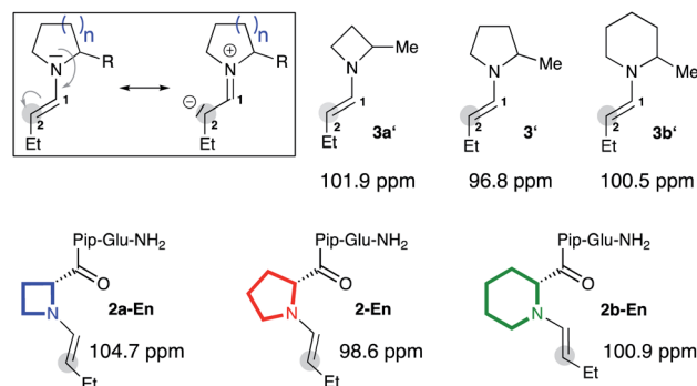
Fig. 2 13 C NMR chemical shifts of C(2) of enamines derived from \alpha -methyl azetidine ( 3a' ), pyrrolidine ( 3' ), piperidine ( 3b' ) and catalysts 2a-En , 2 , and 2b-En in d 6 -DMSO.
