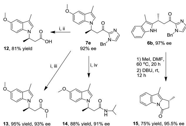
Scheme 2 Synthetic elaboration studies. Reaction conditions: (i) MeI, DMF, 60\text{ }^\circ\text{C} , 20 h; (ii) DBU, \text{H}_2\text{O} , rt, 4 h; (iii) DBU, \text{CH}_3\text{OH} , \text{CH}_2\text{Cl}_2 , rt, 6 h; (iv) DBU, i\text{PrNH}_2 , rt, 12 h.
