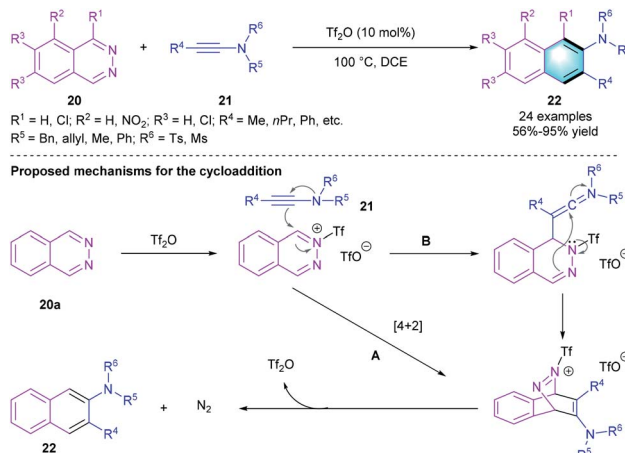
Scheme 5 Tf 2 O-catalyzed [4 + 2] benzannulation to synthesize 2-aminonaphthalenes and 2-aminoanthracenes.
