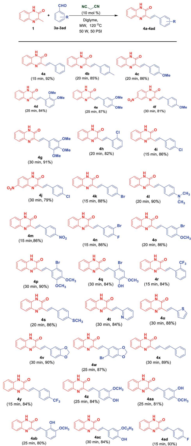
Scheme 3 Substrate scope for synthesis of 3-substituted styrlquinoxalin-2(1 H )-ones 4a–4ad from 3MQ 1 and aryl/hetaryl aldehydes 3a–3ad .
