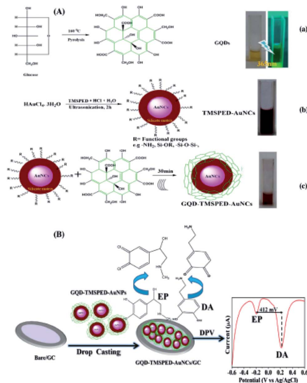
Fig. 10 A schema of the procurement process of (A) GQD-TMSPED-AuNCs nano-composites and (B) electro-chemically concurrent determination of EP and DA. Reprinted with permission. 153 Copyright 2019, Springer.
