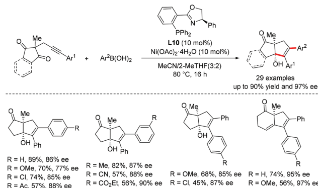
Scheme 30 Ni-Catalyzed enantioselective anti -arylation of alkyne-nitriles with organoboronic acids.
